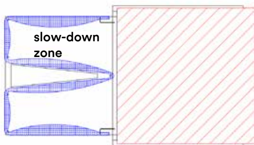
Secondary filter NFE02 with optimally integrated slow-down zone: 400 mm air slow-down zone in two chambers.
