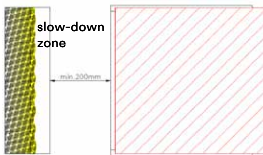
Secondary filtering systems NFEWP02 and NFEWP03: At least 200 mm of air slow-down zone is planned in the construction.
