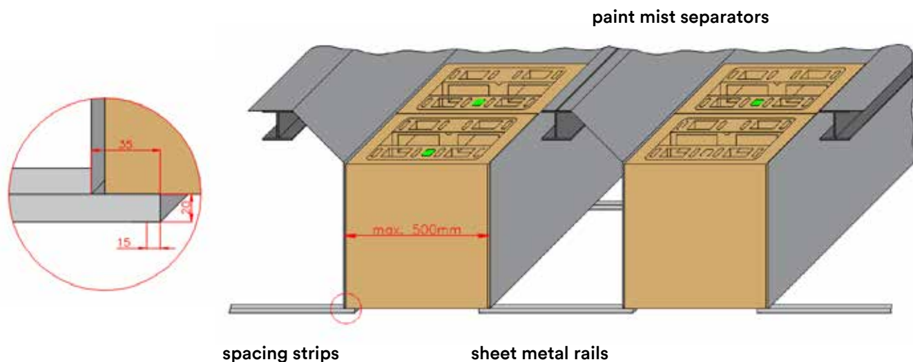
Figure: Proper insertion of the VARIO paint mist separator is illustrated in this angular cross-section: The base and cover of the VARIOS lie against the side walls of the sheet metal rails.
