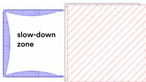
Secondary filter CUBE01 with optimally integrated slow-down zone: 400 mm air slow-down zone in two chambers.
